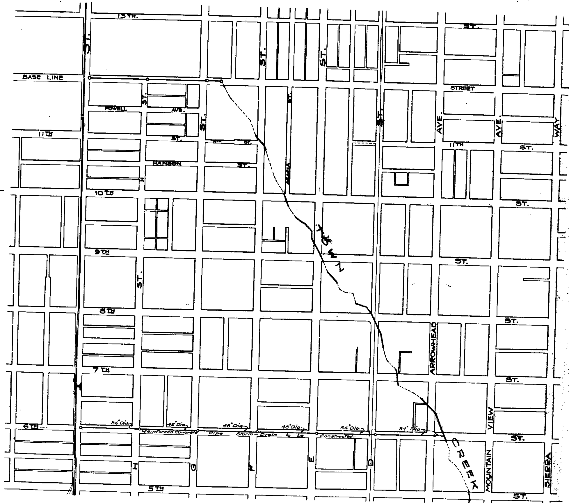
PROPOSED STORM DRAIN ALONG SIXTH ST. AND BASE LINE ST. CITY OF SAN BERNARDINO
